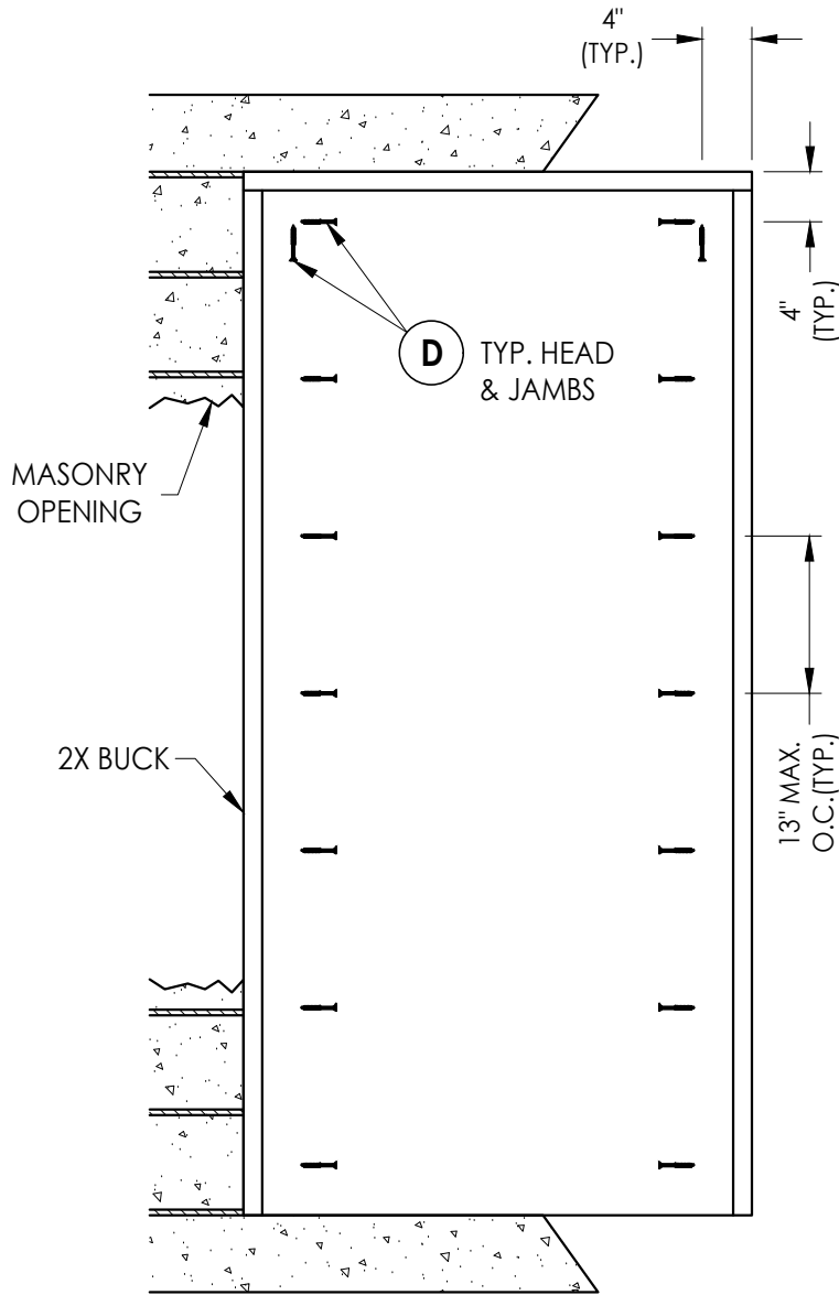
BUCK ANCHORING
