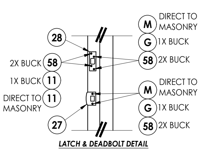
LATCH & DEADBOLT DETAIL
